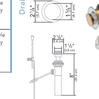
Drain 1 1/2" Drain
