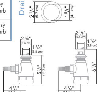
Drain 1 1/2" Drain
