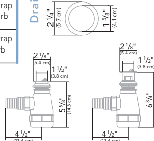
Drain 1 1/2" Drain
