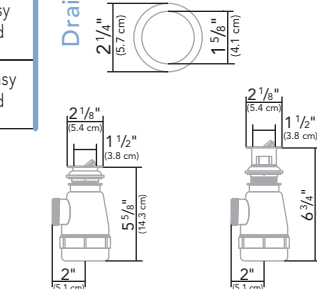
Drain 1 1/2" Drain
