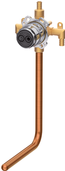
Treysta® G00GS52 Series Tub & Shower Rough-in Valve - Vertical Inputs with Stub-out, without Service Stops
