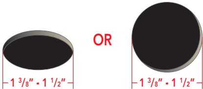
Deck-Mount
